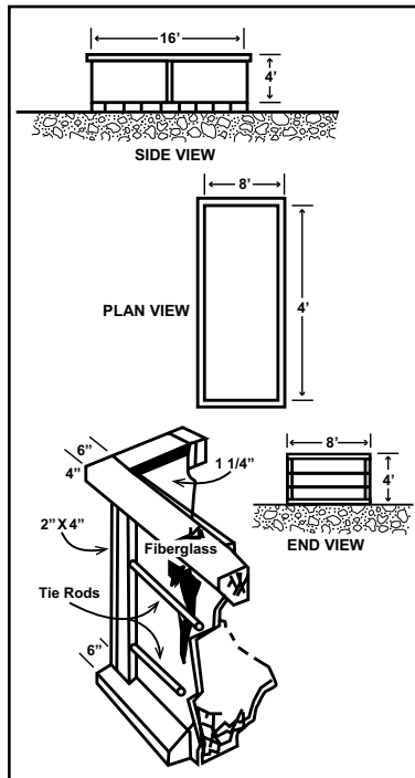
Figure 3. Plywood and fiberglass tank design.
