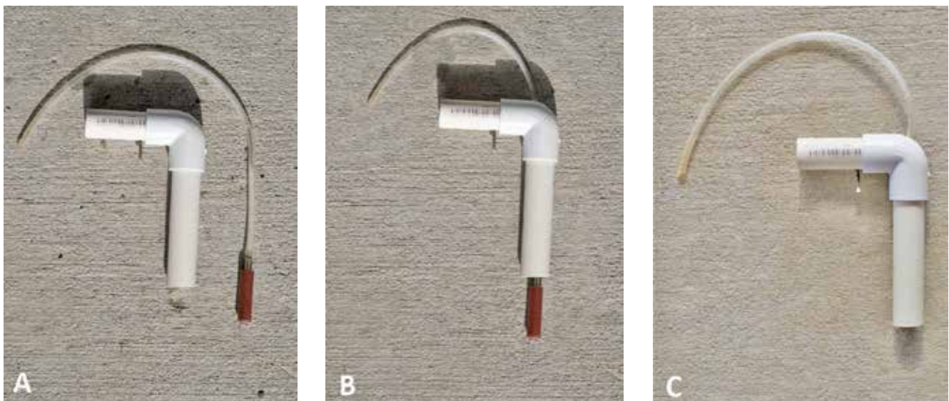
Figure 16. An airlift. (A) “L” shaped airlift with flexible air hose and air stone. (B) The air hose is inserted into the airlift through a hole in the elbow and the air stone attached to the hose. (C) The air-stone has to be pulled up into the airlift for water to be lifted.
