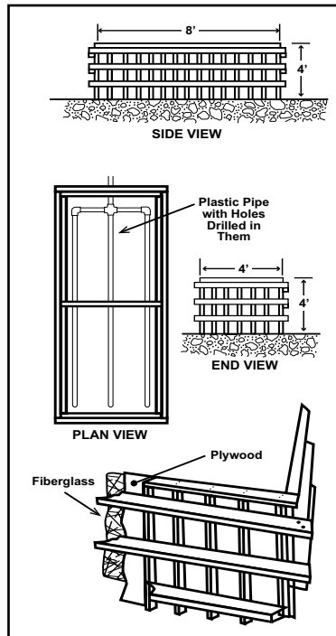
Figure 4. Setting tank design. 2 x 4s and 2 x 6s used instead of tie rods as in Figure 3 (from Jones and Jones, 1988).
