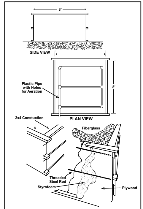
Figure 5. An insulated tank design. Insulation is particularly important if the seawater is heated, to keep heating costs low (from Jones and Jones, 1988).
